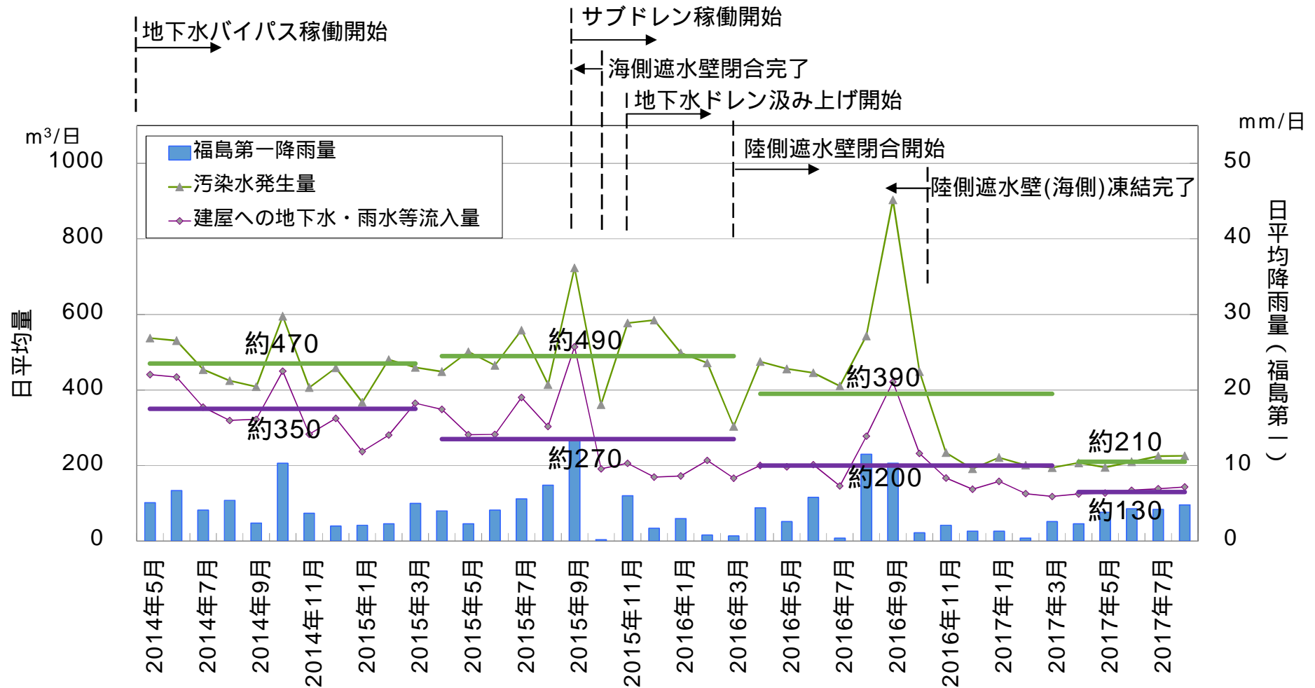
©Tokyo Electric Power Company Holdings, Inc. All Rights Reserved 汚染水発生量のこれまでの低減状況
