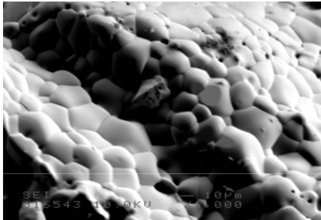
(a)25%Zry-UO 2
