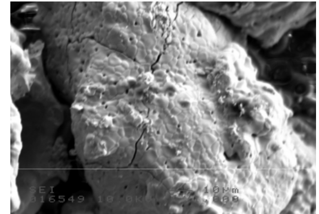
(c)75%Zry-UO 2
