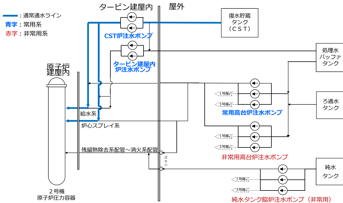
©Tokyo Electric Power Company Holdings, Inc. All Rights Reserved. 原子炉注水設備概略図 (2号機を例示)
