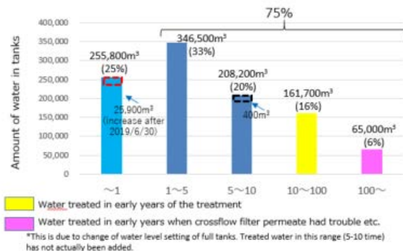
Sum of the ratios of actual concentrations to regulatory standards for 62 nuclides* (other than tritium)
