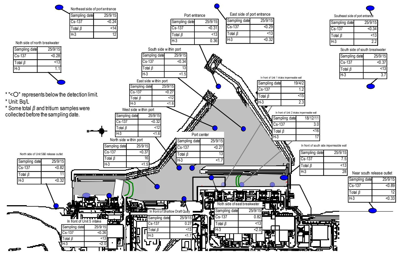
Figure 5: Seawater concentration around the port
