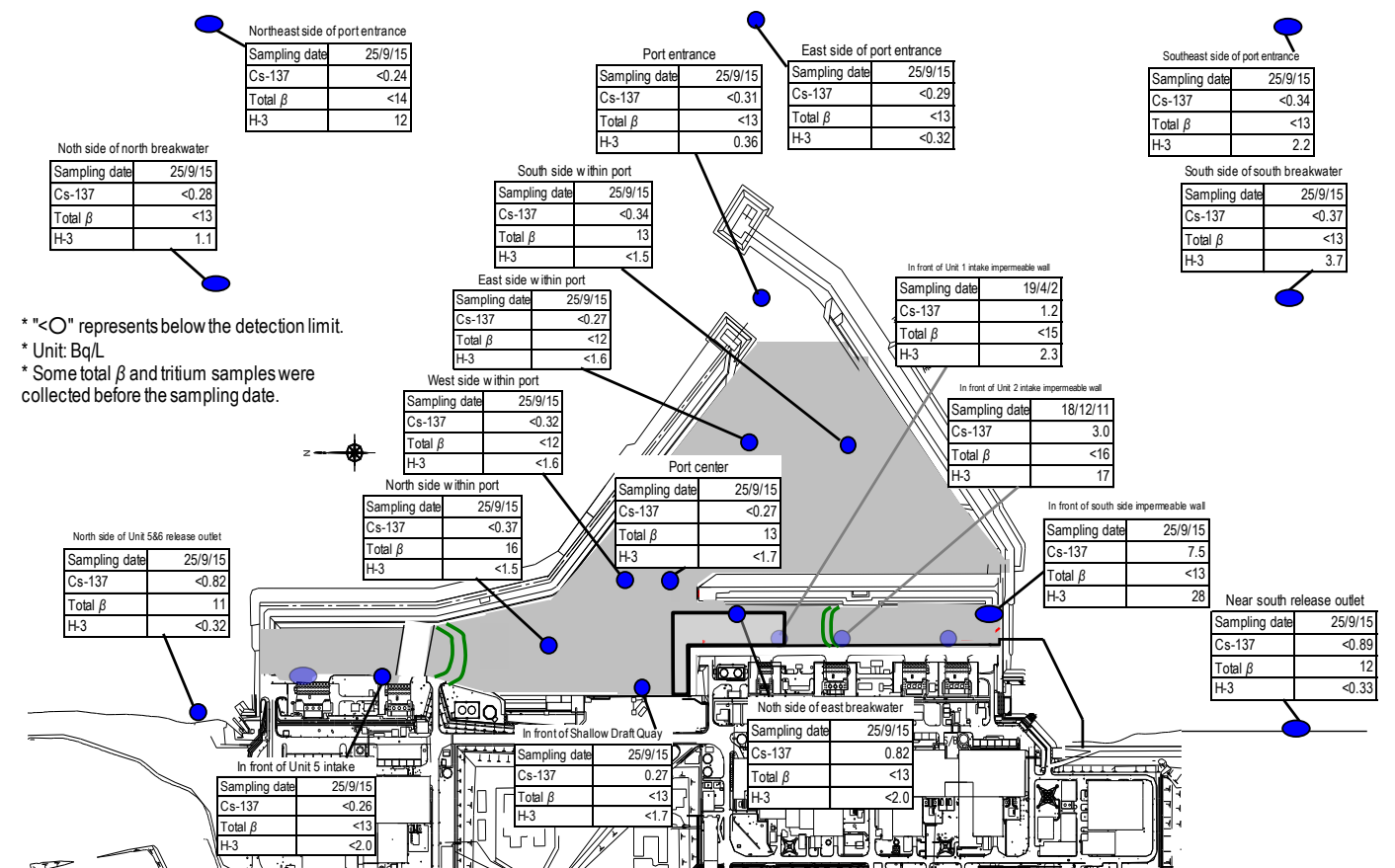
Figure 5: Seawater concentration around the port
