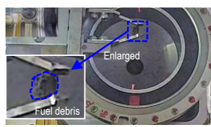
Collecting gripped fuel debris in the transportation box
