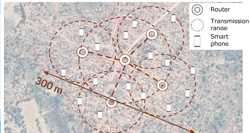
Installation of mesh networks in villages
