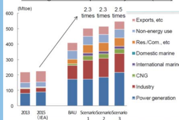
Natural gas demand potential by sector (2030)
