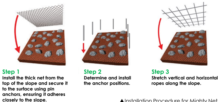
▲ Installation Procedure for Mighty Net
