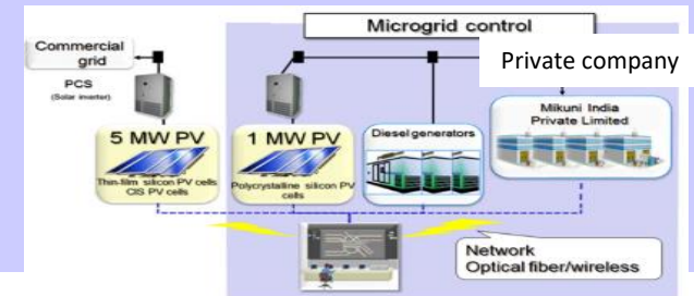
Figure 2. System configuration at Neemrana Industrial Park in Rajasthan
