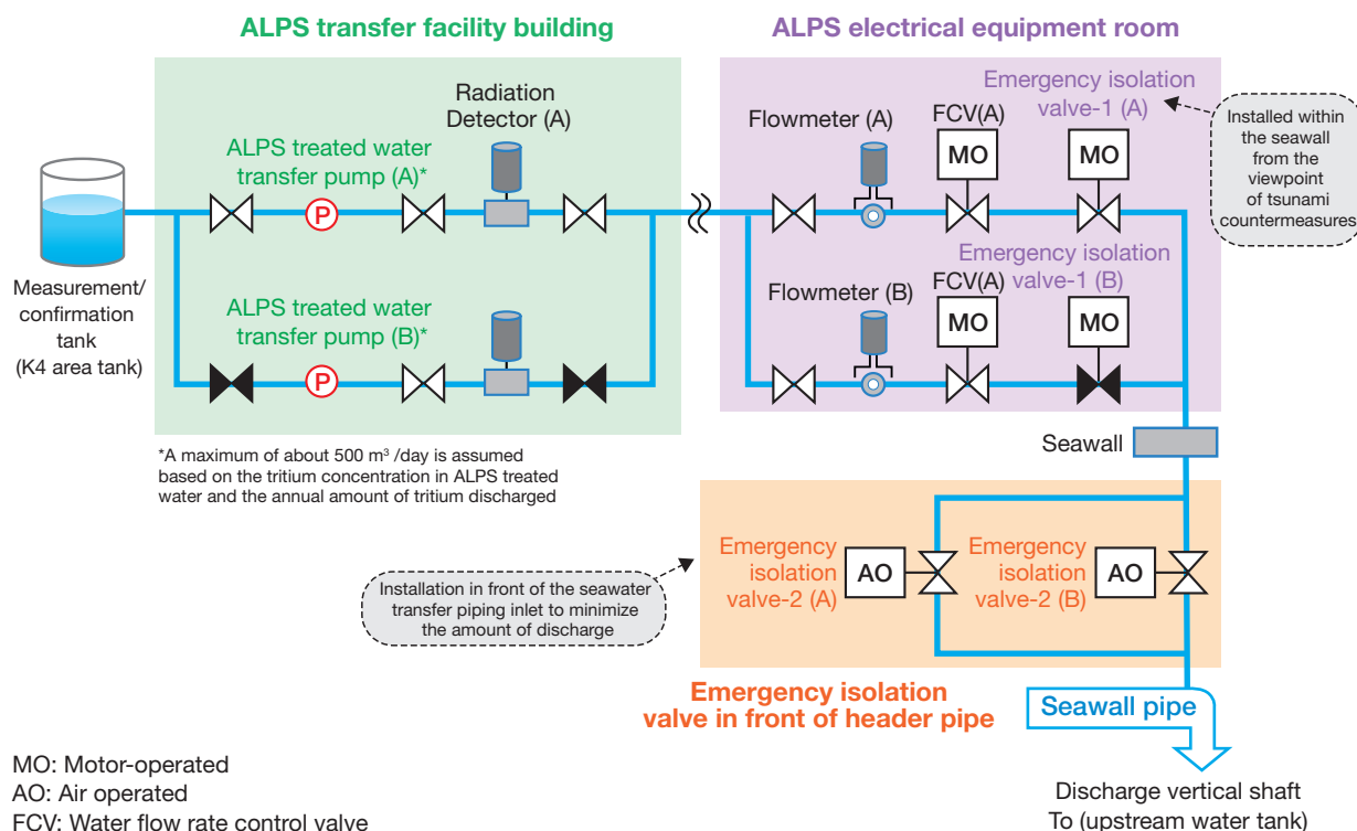
Figure 3.3. Transfer Facility
