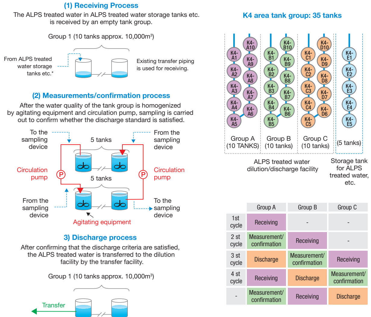
Figure 3.2. Process for receiving, measuring and discharging ALPS treated water
