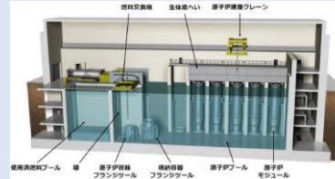
◆ VOYGR (NuScale社)
