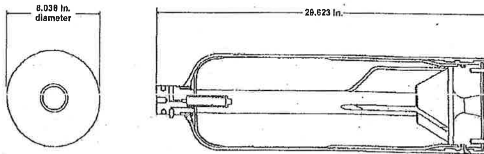
FIGURE 7. NAWCWD Standard Graphite Case Motor
