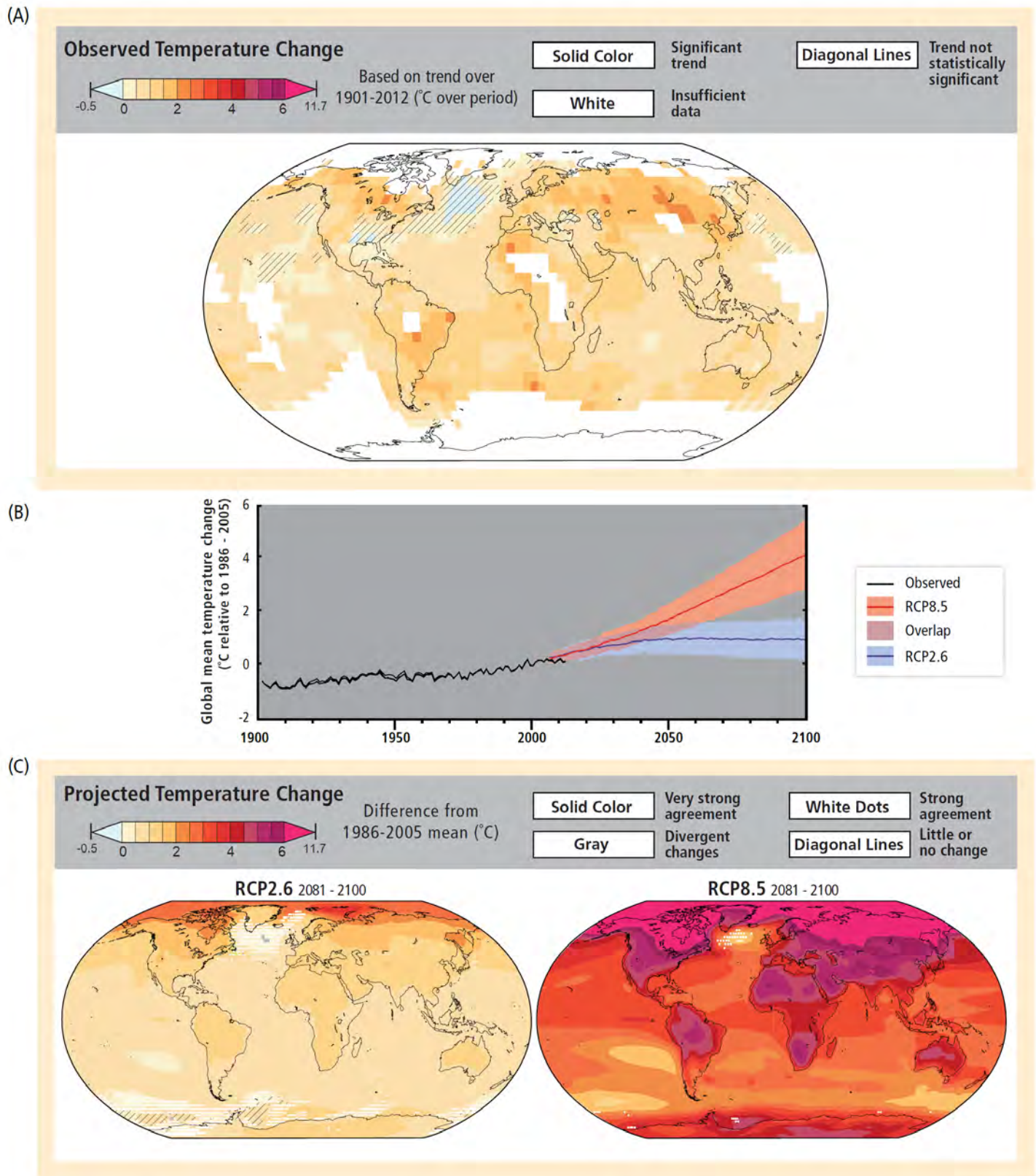
Figure SPM.4.
