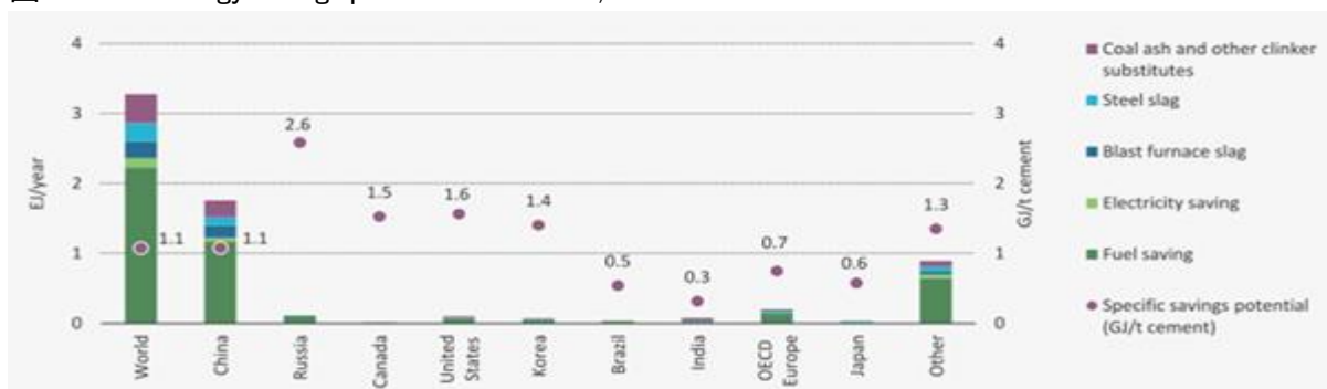
図 Current energy savings potential for cement, based on BATs
